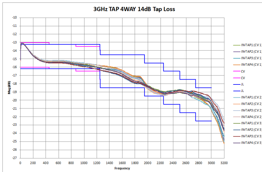
Figure 13: Test data for Tap14 tap loss
