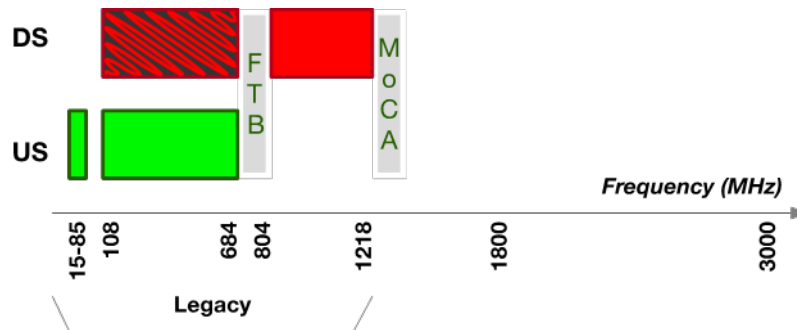
Figure 9: Frequency Plan with Extended FDX
