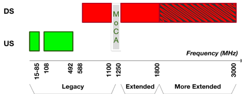
Figure 10: 1.8 GHz Static FDX Frequency Baseline
