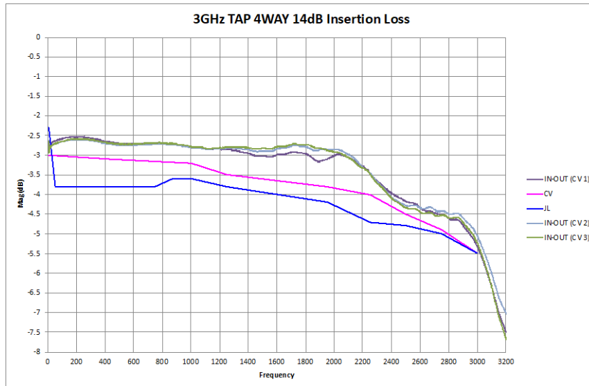
Figure 12: Test data for Tap14 insertion loss
