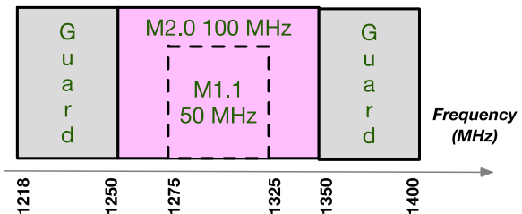
(c) Single Channel with MOCA 1.1 or 2.0 at 1218 MHz
